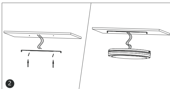
2. Wiring and color temperature adjustment
