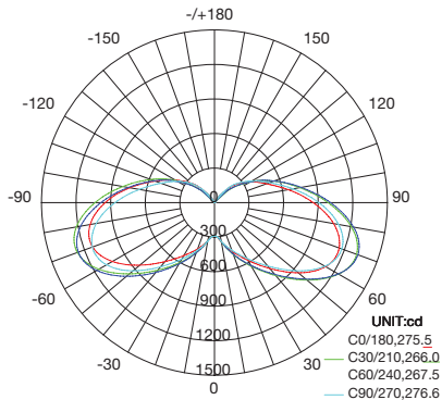
INTENSITY DISTRIBUTION DIAGRAM
