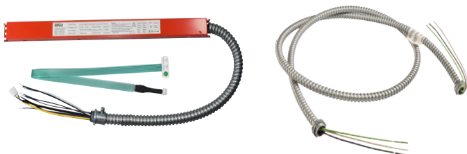
WSD-EMLY15W27-XX 15W Emergency Backup Battery LED Driver
