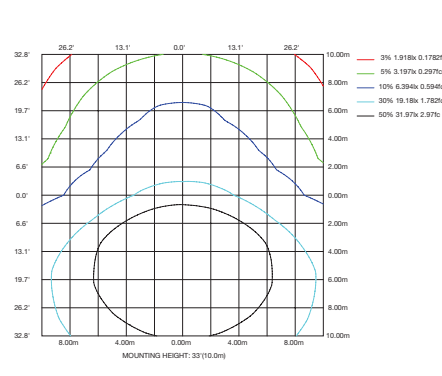
ISOLUX DIAGRAM
