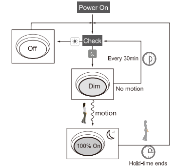
100% on when movement detected, and dims to 10% in long absence. When the natural light level exceeds setpoint off to light, the light will turn off even if when the space is occupied. The light automatically turns on at 10% when natural light is insufficient (no motion).
