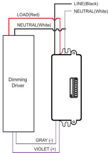
Dimming Driver
