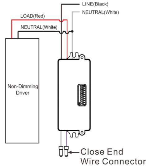
Non-Dimming Driver
